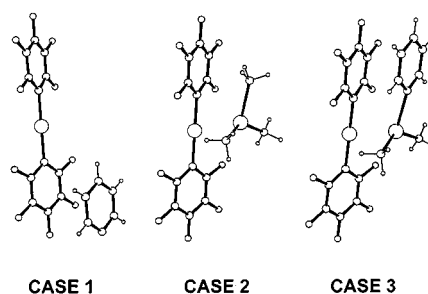
Figure 2. The assumed structures of the theoretical models, (a): [\text{Au}(\text{C}_6\text{F}_5)_2] \cdots \text{Py} CASE 1; (b): [\text{Ag}(\text{NH}_3)_3] \cdots [\text{Au}(\text{C}_6\text{F}_5)_2] CASE 2; (c): [\text{Ag}(\text{NH}_3)_2(\text{Py})] \cdots [\text{Au}(\text{C}_6\text{F}_5)_2] CASE 3
