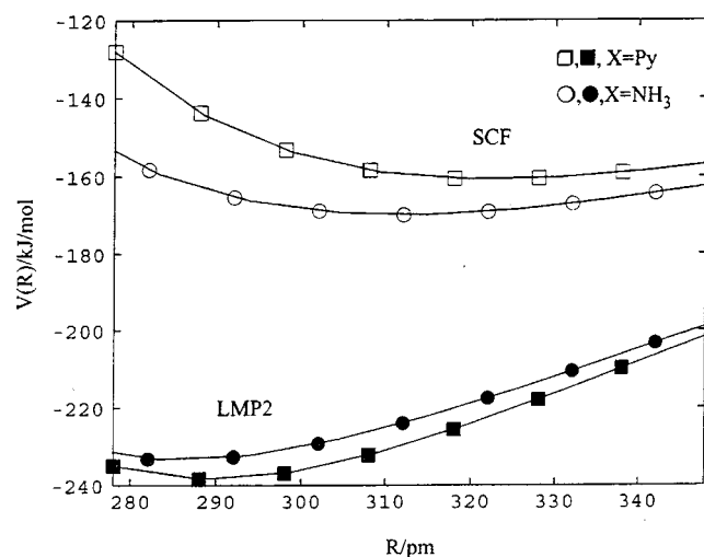
Figure 3. Interaction energy curves for the [\text{Au}(\text{C}_6\text{F}_5)_2] \cdots [\text{XAg}(\text{NH}_3)_2] ( \text{X} = \text{NH}_3, \text{Py} ) interaction calculated at the SCF and LMP2 levels
